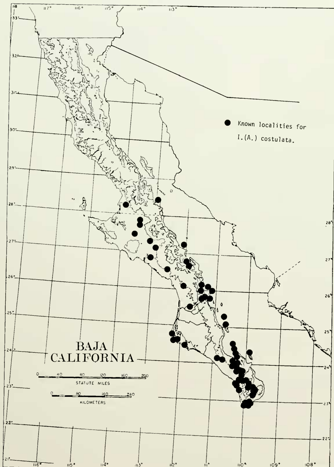
Figure 16. Known distribution of Ichthiacris ( Aryphacris ) costulata (circles).
